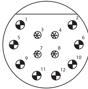
3212 (12 #16 AWG)
